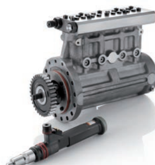
COMMON-RAIL SYSTEMS
